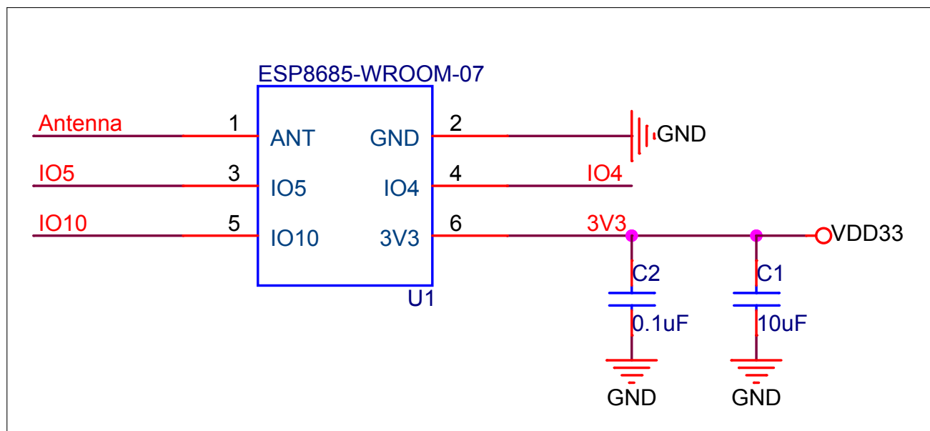
Figure 5: Peripheral Schematics
