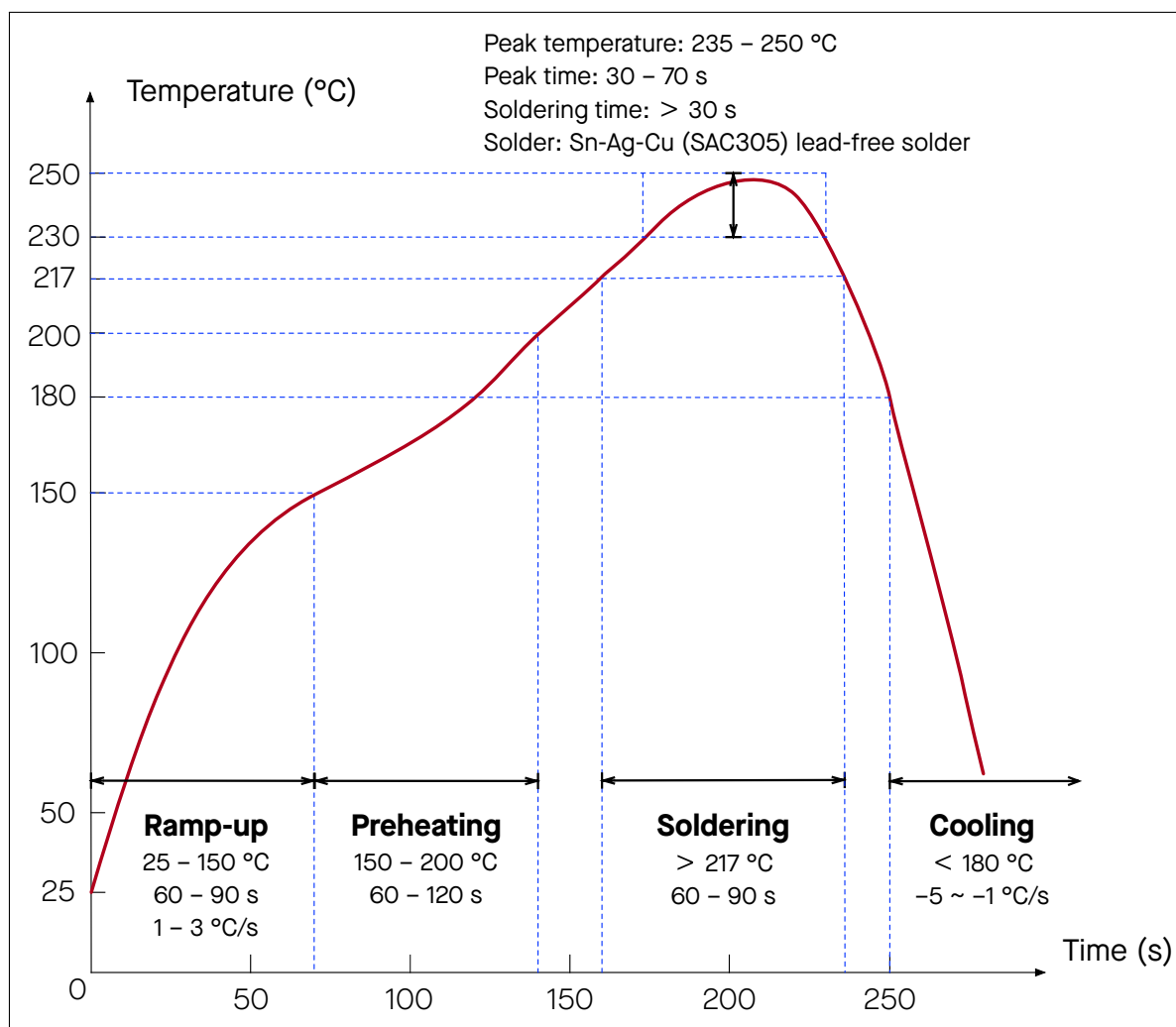
Figure 9: Reflow Profile
