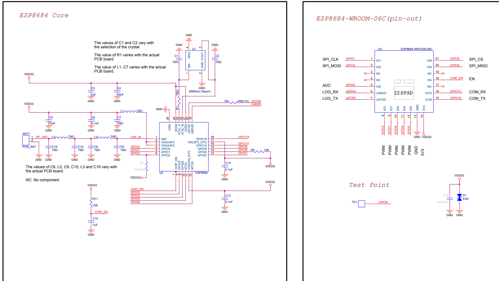
Figure 4: ESP8684-WROOM-06C Schematics
