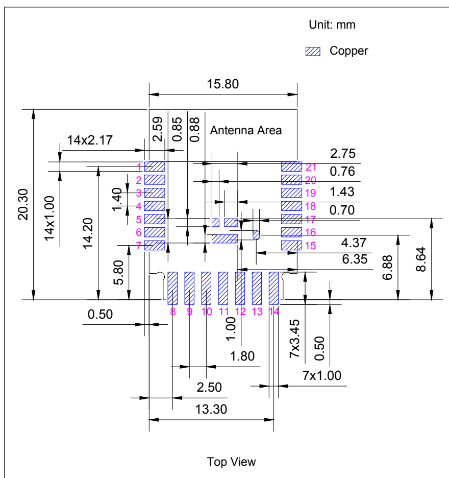
Figure 7: Recommended PCB Land Pattern for SMD Soldering
