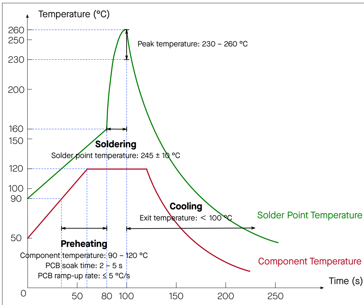
Figure 10: Wave Soldering Profile
